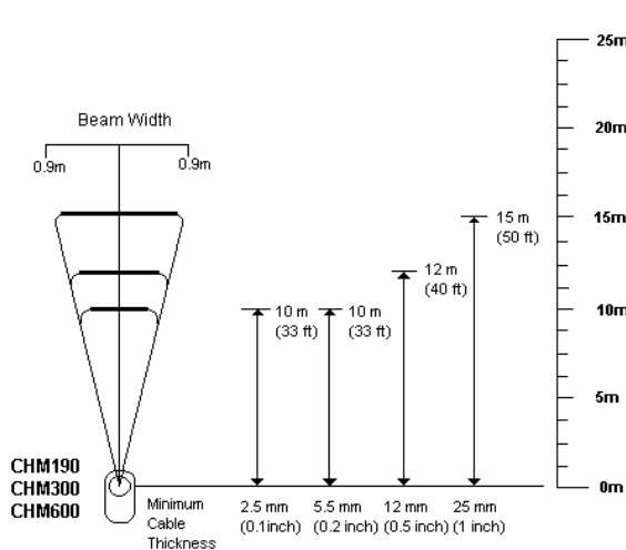
CHM Range versus Cable Thickness
